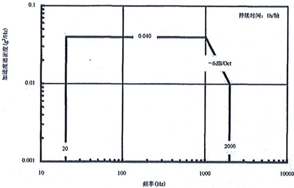
Figure 1 Vibration Spectrum
